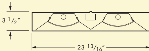
2 T5 or T8 lamps
