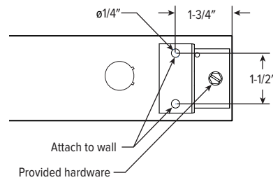
FIG G.3.5 BACKVIEW
