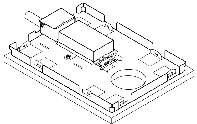
FIG 5.1 NEW CONSTRUCTION
