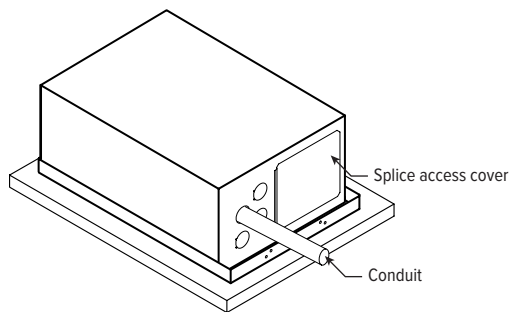
FIG 4.2 IC MOUNTING
