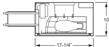
Single fixture, standard arm mount: EPA: 1.59/Weight: 35 Lbs.
