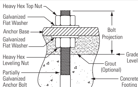
BOLT PROJECTION DETAIL
