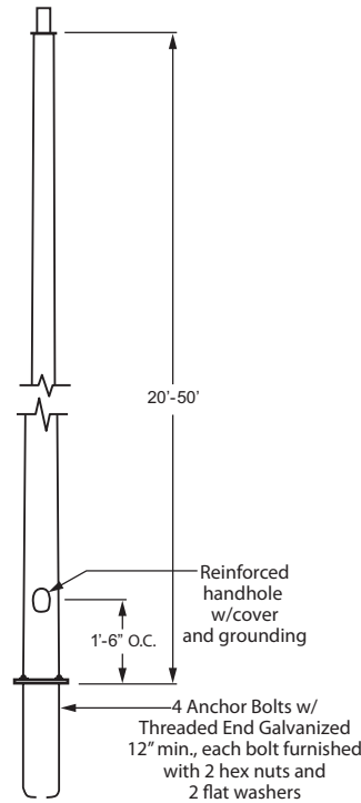
Pole Detail
