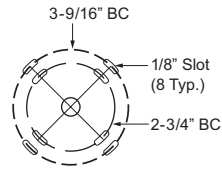
BOLT CIRCLE PATTERN DETAIL
