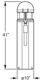
Shown with VG and DT Weight: 188 Lbs.
