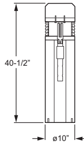
Shown with HG and FT Weight: 200 Lbs.
