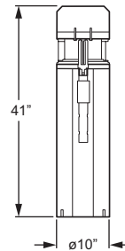
Shown with VG and FT See back for additional cross-sections and fixture weights
