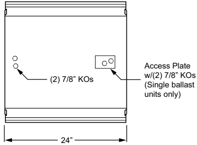
2 X 4 - 2 & 4 LAMPS
