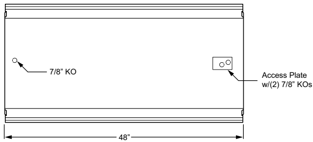
2 X 4 - 2 & 4 LAMPS
